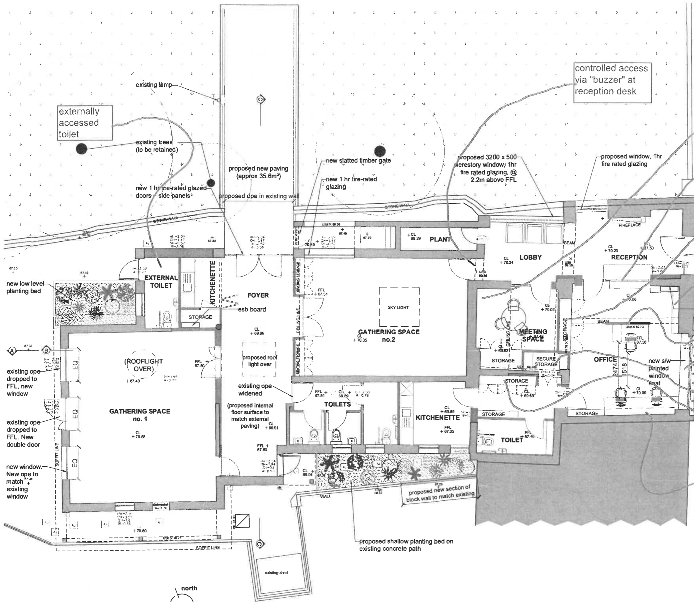
Ground floor - PROPOSED 1:100
